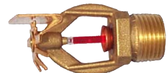
QUICK RESPONSE HORIZONTAL SIDEWALL
